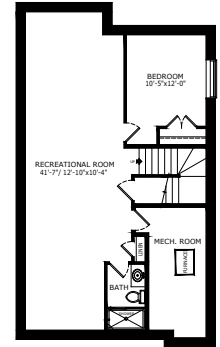
1 BEDROOM 'LEGAL SUITE' 816 SQ FT
